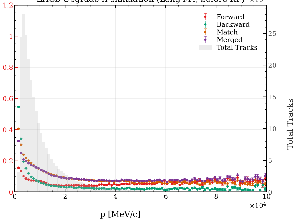
LHCb Upgrade II simulation (Long MT, before KF) \times 10^4
